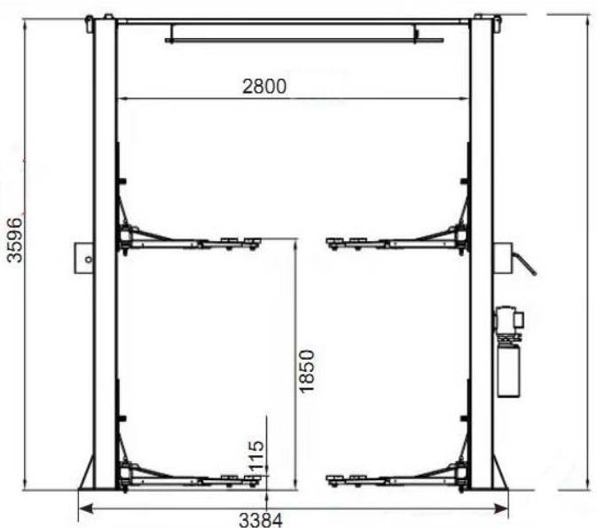
LJCC Layout Diagram
