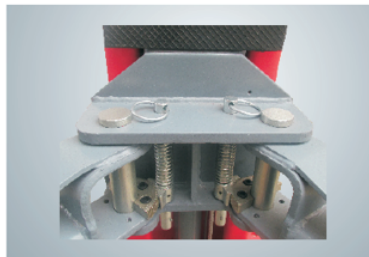
Arm Locking mechanism adopt thicker top rod and widetooth block, lift the vehicle more reliably
