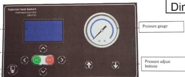
Control panel
